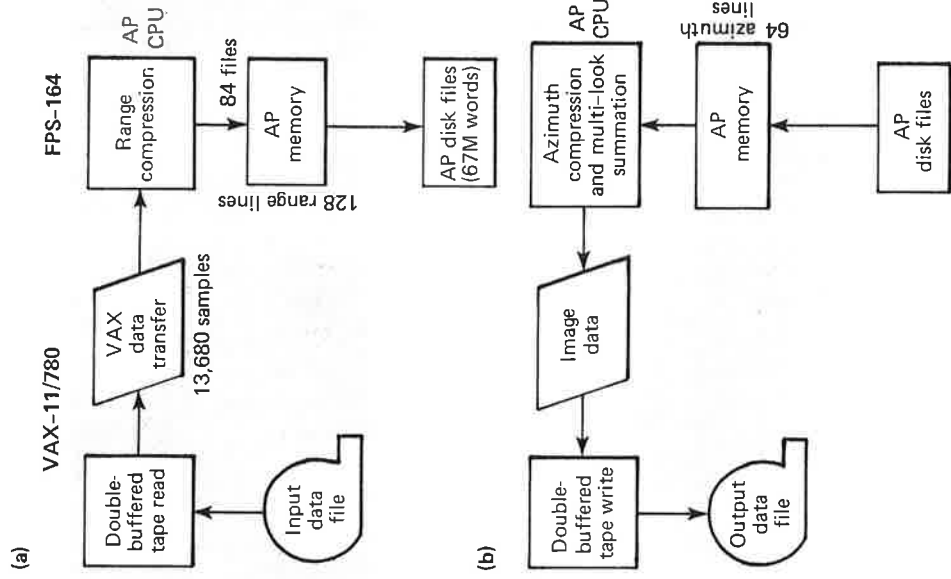
Figure 9—Data flow during (a) range compression and (b) azimuth compression. AP is the FPS-164 attached processor.
