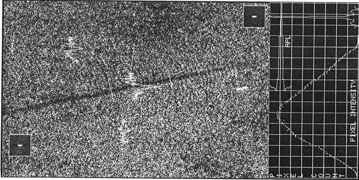
Figure 11 —Seasat English Channel scene, showing range structure in ship wake and processor range and azimuth resolution and sidelobe structure as measured by noise autocorrelation.
